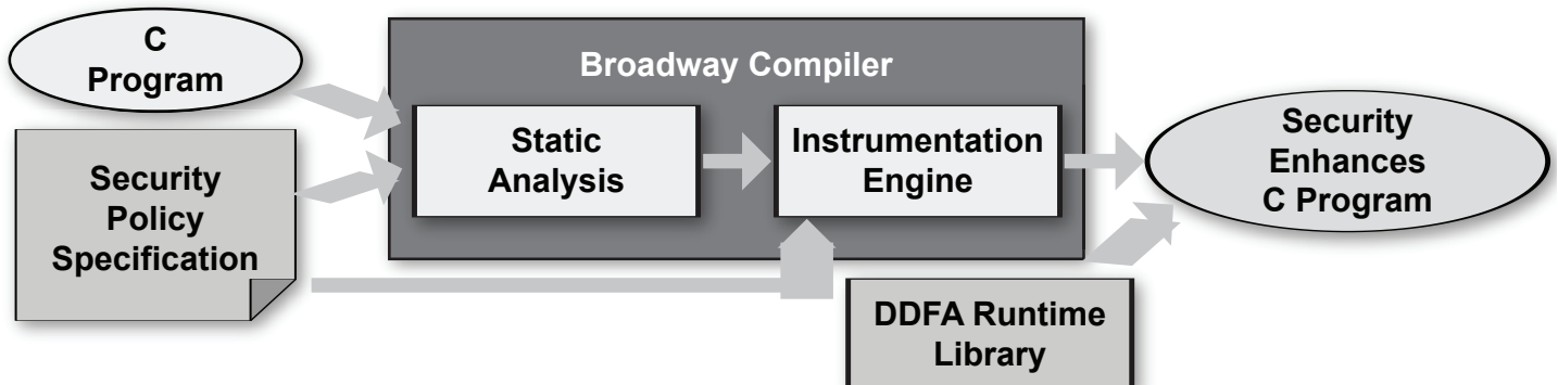
Figure 1: Overall Architecture of DDFA System
